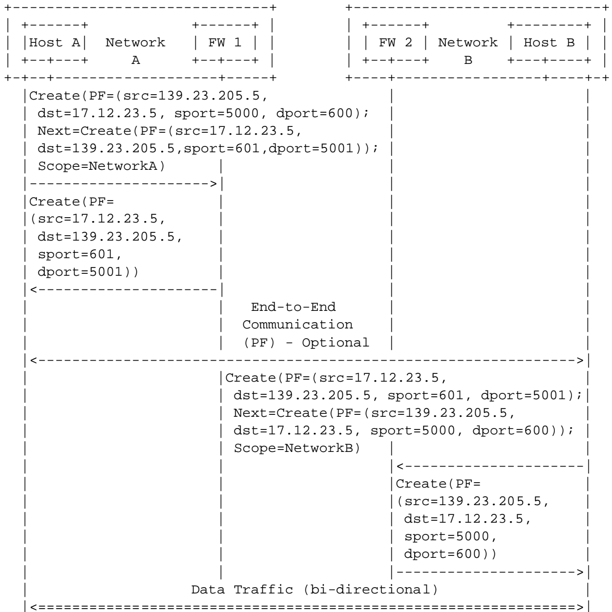
Figure 12: Sender-Initiated Firewall Signaling only at the Access Network
