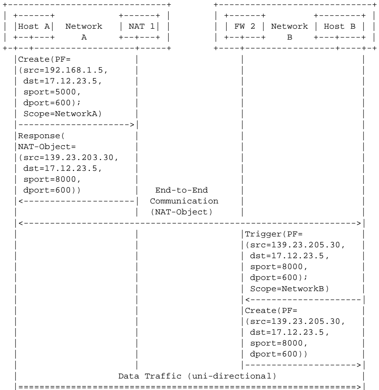
Figure 13: Sender-Initiated NAT and Firewall Traversal within the Access Network
