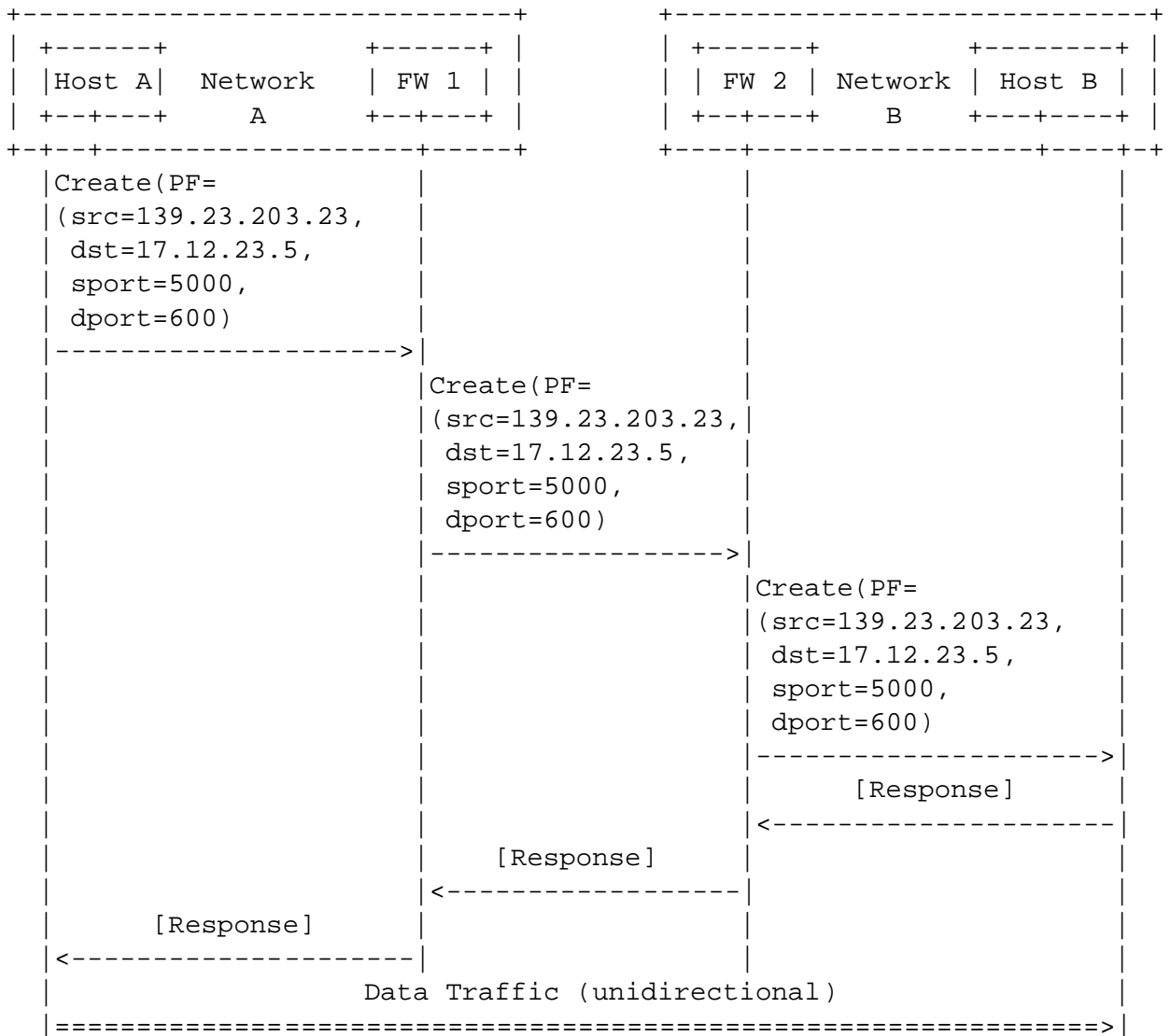
Figure 8: Sender-Initiated Message Flow with Firewalls
