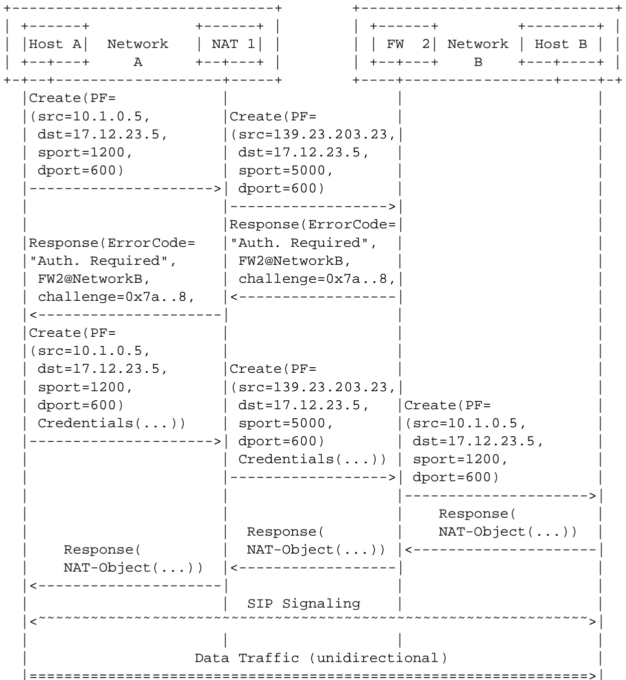
Figure 10: Sender-Initiated Message Flow with a Firewall and a NAT
