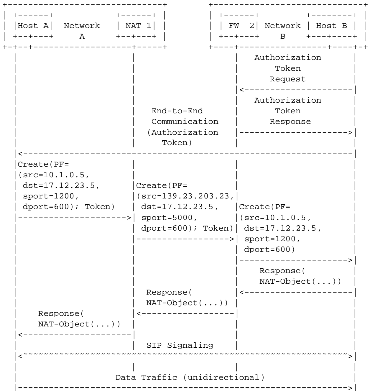
Figure 11: Sender-Initiated NAT/Firewall Traversal with Authorization Token
