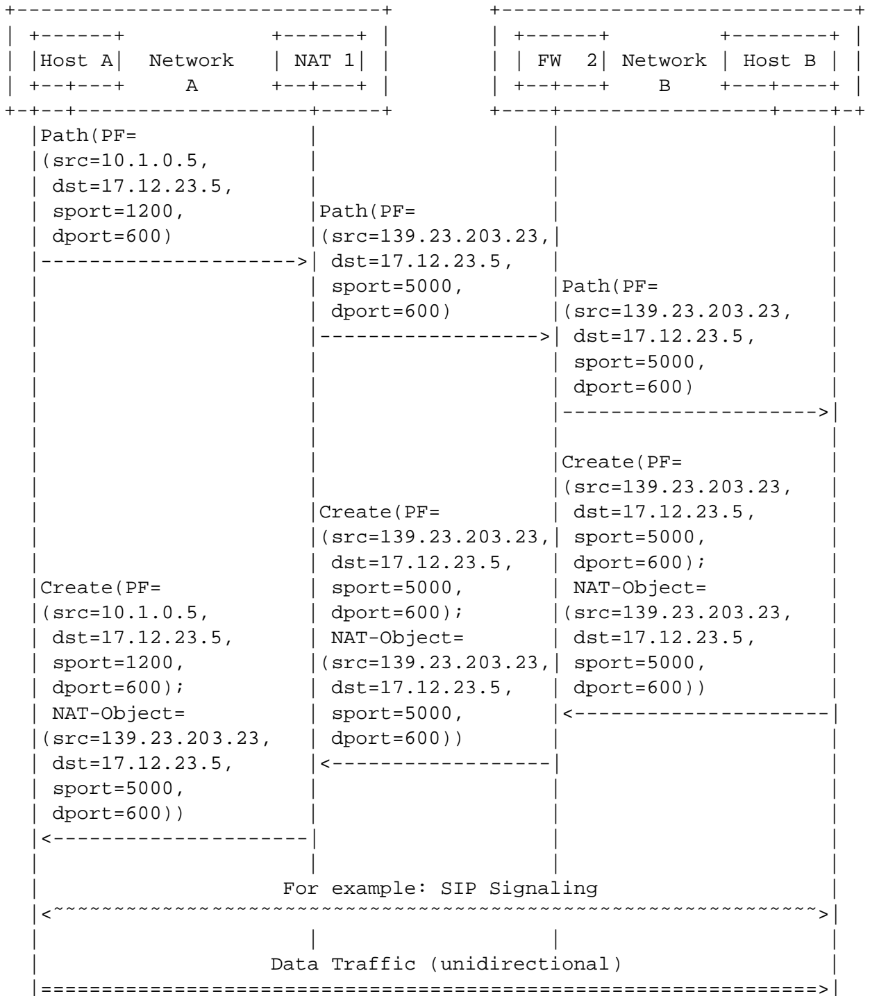
Figure 9: Receiver-Initiated Message Flow with a Firewall and a NAT
